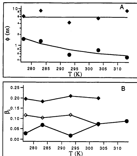
FIGURE 11: Temperature dependence of barycenters (A) and integrated amplitudes (B) as obtained from the correlation time spectra of GR in 50 mM potassium phosphate buffer at pH 7.0: \blacklozenge , integrated amplitude and barycenter of process associated with energy transfer; \bullet , integrated amplitude and barycenter of process associated with restricted motion; \diamond , limiting anisotropy.
