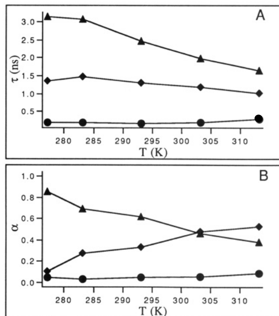
FIGURE 3: Temperature dependence of barycenters (A) and fractional contributions (B) of the lifetime classes in LipDH-AV in 50 mM potassium phosphate buffer at pH 7.0.
